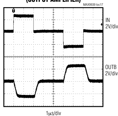
RECOVERY FROM INPUT OVERLOAD (OUTPUT AMPLIFIER)
