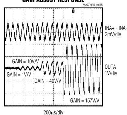
GAIN ADJUST RESPONSE
