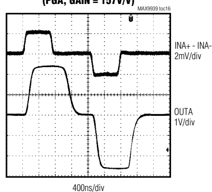
RECOVERY FROM INPUT OVERLOAD (PGA, GAIN = 157V/V)
